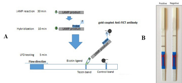
Figure 5. Lateral flow Dipstick Las-LAMP Evaluation. (A) Lateral Flow Dipstick Las-LAMP procedure: LAMP reaction is performed using a biotinylated FIP primer. After 30 minutes of initial incubation at 65°C, a specific FITC-labelled probe is added to the reaction mixture and incubated for another 10 minutes at the same temperature. This step produces a dual labeled LAMP product. Finally, detection buffer containing Rabbit Anti-FITC antibodies coupled with colloidal gold is mixed with the reaction mixture, and the LFD strip is inserted into the tube. In a positive reaction, double labeled LAMP products migrates with the buffer flow and are retained at the Test Band by a biotin ligand. The gold coupled Anti-FICT antibody binds to the FITC molecule at the probe and a dark red band develops over the time. In the case of a negative reaction no products are generated and such process does not have place. An Anti-Rabbit antibody at the Control Band retains some of the unbound gold-conjugated antibody and produces a Control Band that should be always visible. (B) Evaluation of results using the Lateral Flow Dipstick device
