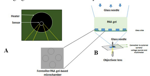
Figure 4. A) Microheater pattern: The microheater system comprised of circular heater and a temperature sensor B) Experimental setup with microscopic view of PAA gel-based microchamber: sample solution was initially deposited on a glass slide, printed with the microheater. The PAA gel-based microchamber was then placed above the sample solution and a glass needle was lowered to press the upper surface of the gel against the glass slide. This way, only one or two DNA templates would be trapped within a single microchamber. Finally, SYBR green II dye was applied to cover the external of the PAA gel, keeping it hydrated in order to retain its structure and encapsulation capability. The microchambers located within the circumferential region bounded by the heater pattern were observed
