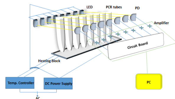
Figure 1. Block Diagram of the Turbidimeter. Eight PCR tubes can be fixed between eight LED and PD. The tubes are heated to the optimum temperature for LAMP reactions (60-65±0.5°C) by a heating block that is designed to avoid blocking the light path. Each light (650 nm; 2 mm I.D.) emitted by eight light emitting diodes (LED) passes through the PCR tube and illuminates the photodiodes (PD) opposed to the LED. The mean optical path length is about 2.5 mm. AC, alternating current; DC, direct current; LED, light emitting diode; PD, photo diode; PC, personal computer
