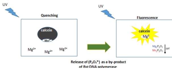
Figure 6. Principle of Detection Using Calcein. In the DNA amplification reaction by Bst DNA polymerase, pyrophosphate ions are released as a by-product from dNTPs. The calcein in the reaction mixture initially combines with manganous ion (Mn 2+ ) and remains quenched. By preceding the reaction, manganous ion is deprived of calcein by the produced pyrophosphate ions (P 2 O 7 4- ), which lead to fluorescence emission. Consequently, the free calcein is apt to combine with magnesium ion (Mg 2+ ) in the reaction solution and it corroborates the fluorescence emission
