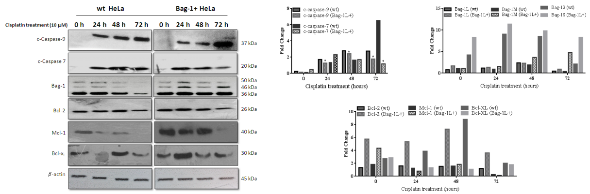
Figure 4. Cisplatin induced Apoptosis Via Modulating Caspases and Bcl-2 Family Members was Observed by Immunoblotting. Cells were seeded at 1 \times 10^6 density in 60mm plates and treated with Cisplatin for 24, 48 and 72h. A total 30 \mu g of protein lysate was loaded in 12% SDS page gel. \beta -actin was performed as a loading control. Image J data analysis for immunoblotting assay was given as column graphs for each protein in wt and Bag-1L+HeLa cells
