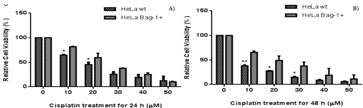
Figure 1. Cisplatin Decreased the Cell Viability in a Dose and Time Dependent Manner in Wild Type (wt) and Bag-1L Stable Transfected HeLa Cells. Cells were seeded at 1 \times 10^4 density and treated with various concentrations of Cisplatin (0-50µM) for 24 and 48h (A-B). The bar histograms represent the mean±SD of four independent trials with at least four replicates. A) p < 0.0001 , B) p < 0.0001 each result was compared with the untreated control cells by using Bonferroni's ANOVA 95% multiple comparison test)
