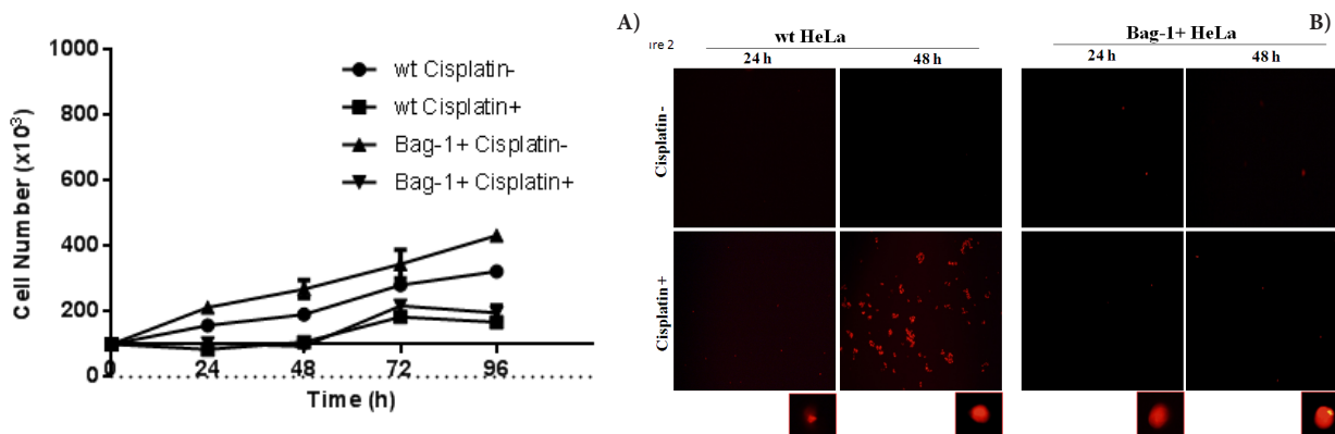
Figure 2. A) Bag-1L Stable Overexpression Enhanced the Protection Effect Against Cisplatin in HeLa Cells Proliferation Rates. wt and Bag-1L+ cells were seeded at 1×10 6 density in 6-well plates and treated with 10μM Cisplatin for 24,48,72 and 96h, According to the time points, cells counted each day for 4 days using trypan blue dye exclusion assay. Lines represent unstained viable cell numbers and the means±SD of three independent trials with at least four replicates; B) Bag-1L Stable Transfection Decreased Dead Cell Number in Cisplatin-induced Apoptosis in wt and Bag-1L+HeLa Cells. Cisplatin-treated apoptotic cells were determined as red dots by PI staining. Images were taken at 200× expansion of cells
