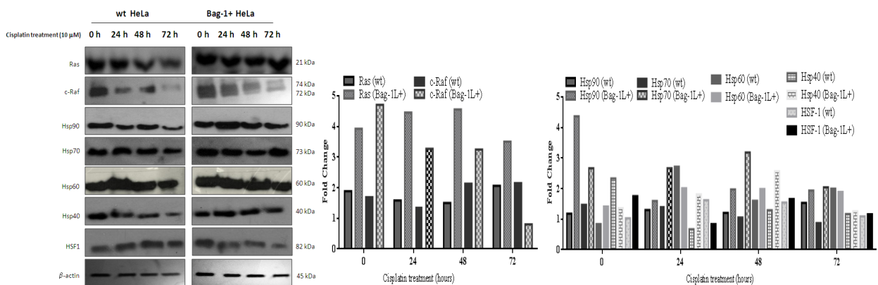
Figure 5. The Effect of Bag-1L Stable Transfection on Oncogenes and Heat Shock Proteins in wt and Bag-1L+HeLa Cells was Observed by Immunoblotting. Cells were seeded at 1 \times 10^6 density in 60mm plates and treated with Cisplatin for 24, 48 and 72h. A total 30 \mu g of protein lysate was loaded in 12% SDS page gel. \beta -actin was performed as a loading control. Image J data analysis for immunoblotting assay was given as column graphs for each protein in wt and Bag-1L+HeLa cells
