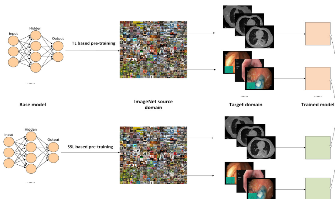
Figure 2. The Basis Models are Pre-Trained with TL and SSL Separately and Fine-Tuned to the Same Datasets [4].
