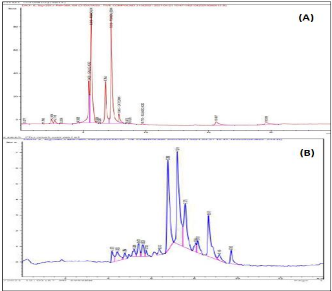
Chromatogram of sonicated Punica granatum peel sample (B) compared to standard phenolics (A)
